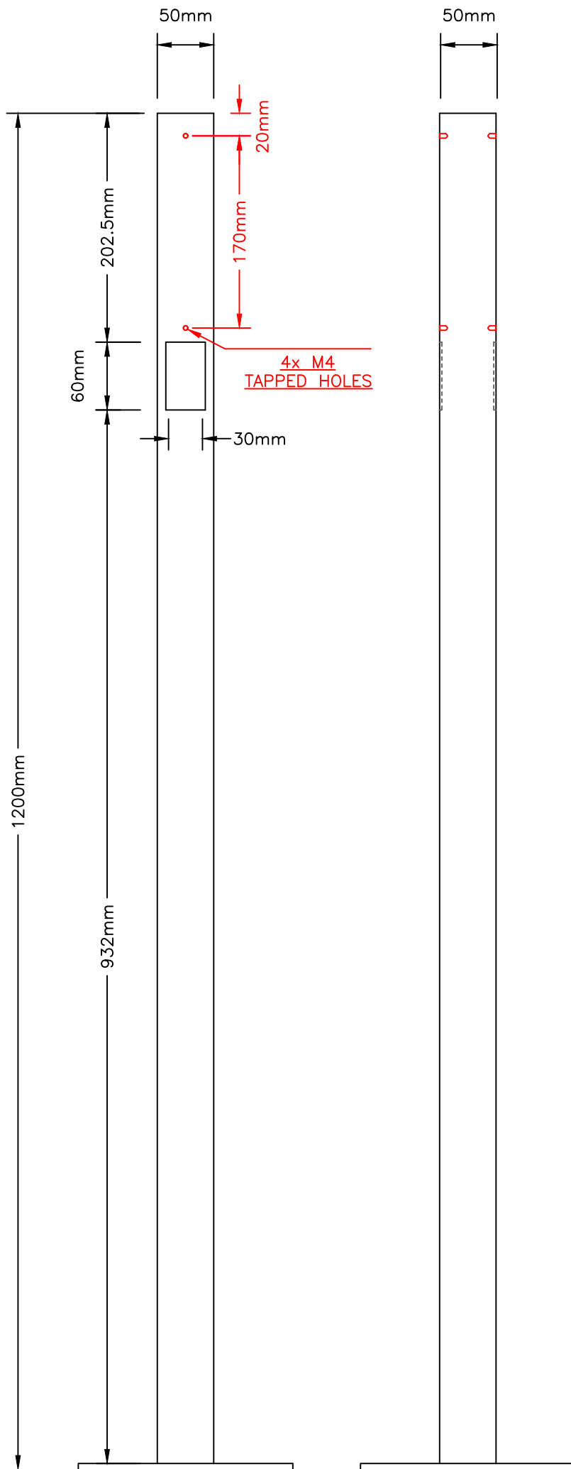
FRONT/REAR VIEW
